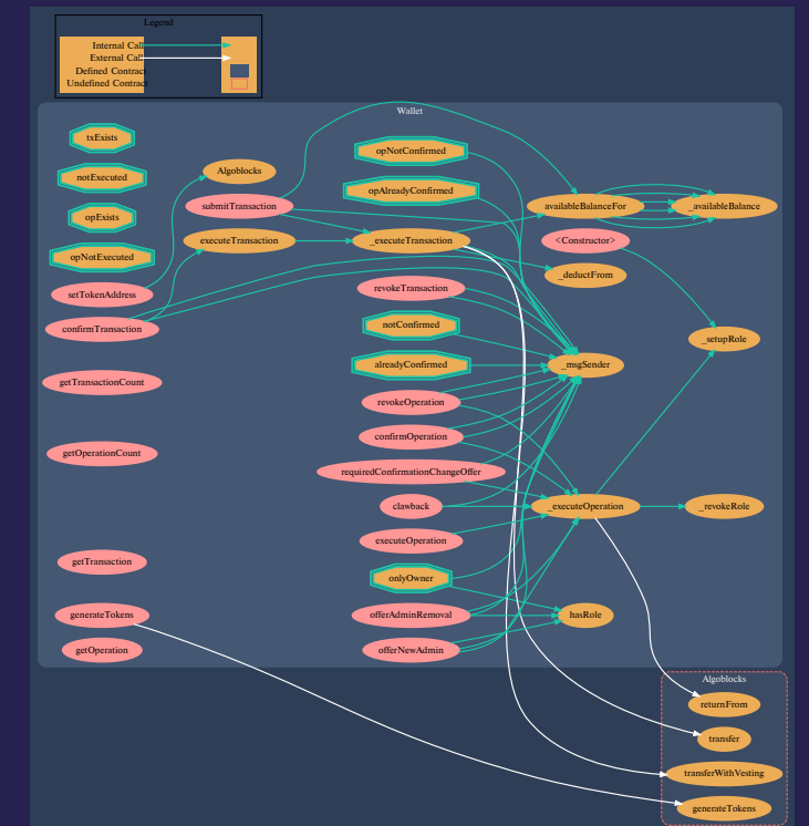
Pic. 1.2 Wallet.sol
