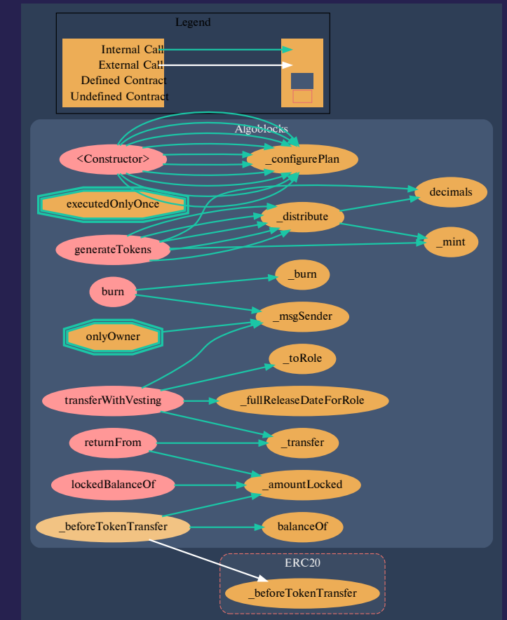
Pic. 1.1 Algotricks.sol
