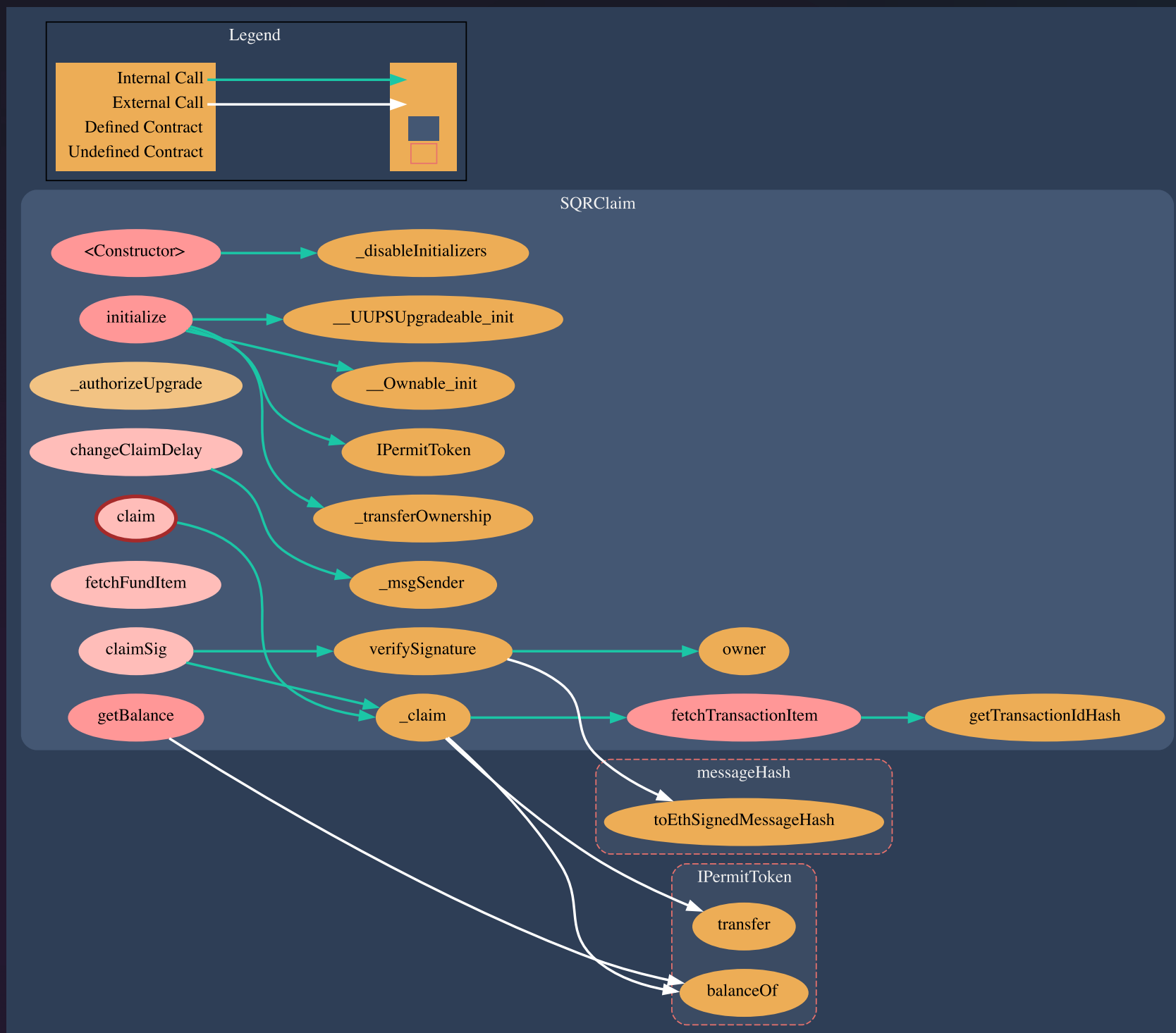
pic.2.1 SQRClaim
